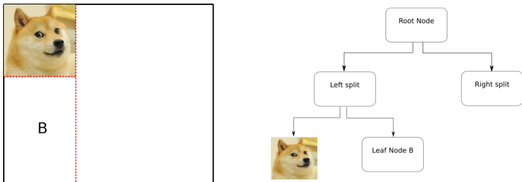
After one iteration of inserting a 2D area into the kDTree we'd get the following tree
