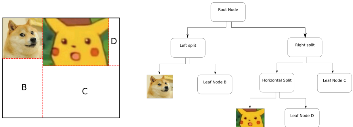
The second 2D area to add is too large for the left split area, and is instead added to the right child node, which is further split, giving us node C
